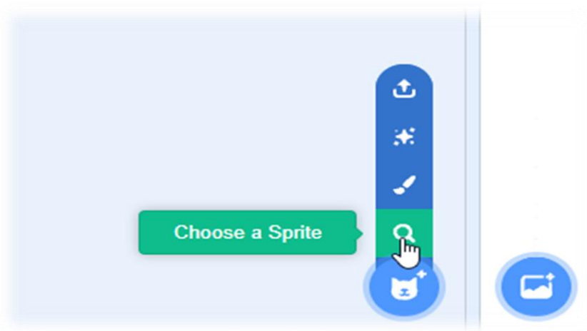
Figure 21: Insert Sprite
