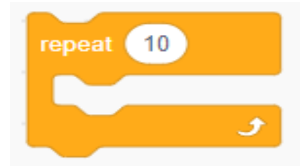
Figure 36: Repeat block
