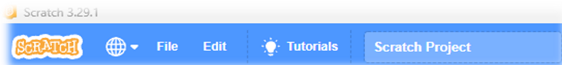
Figure 2: Menu Bar
