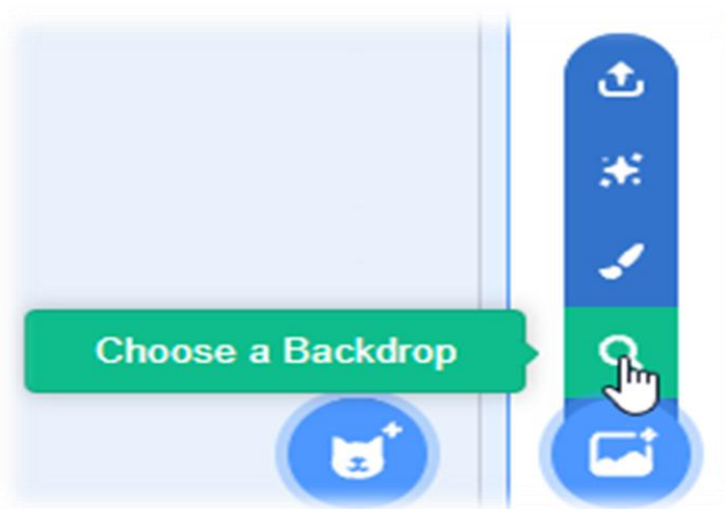
Figure 13: Insert Backdrop
