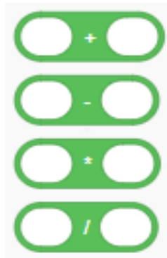
Figure 59: Mathematical Operators
