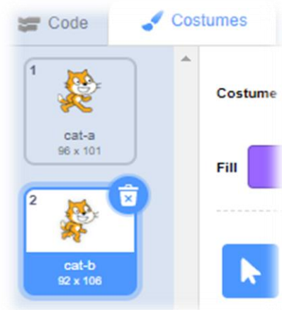
Figure 13: Cat Costumes
