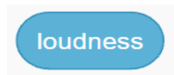
Figure 52: Loudness block
