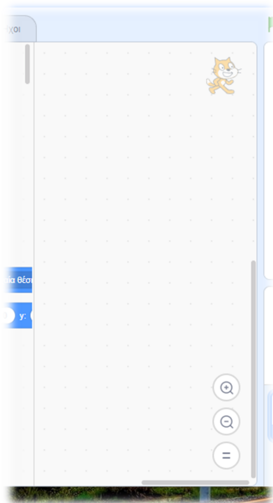
Figure 6: Code Area
