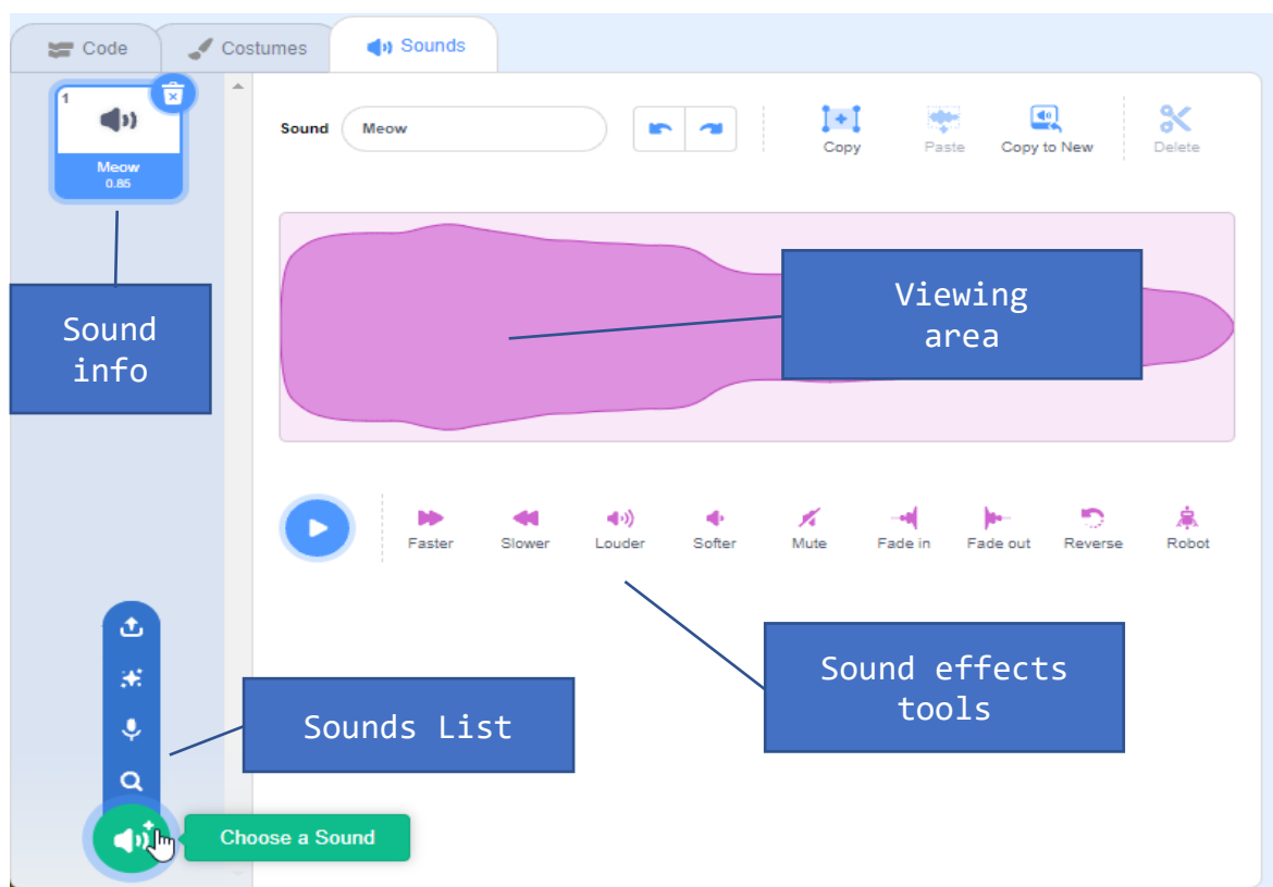
Figure 9: Sounds tab
