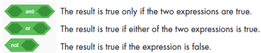
Figure 62: Logical Operators
