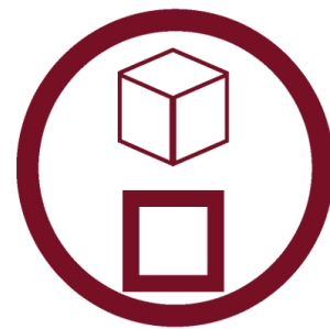
ABSTRACTION
