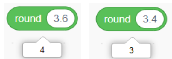
Figure 66: Round block
