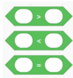
Figure 61: Relational Operator
