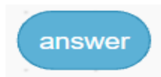
Figure 46: Answer block
