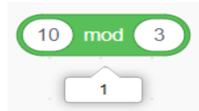
Figure 65: Mod block
