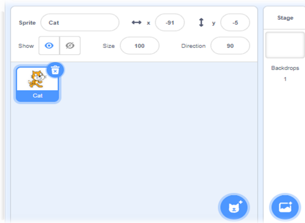
Figure 4: Sprite Pane
