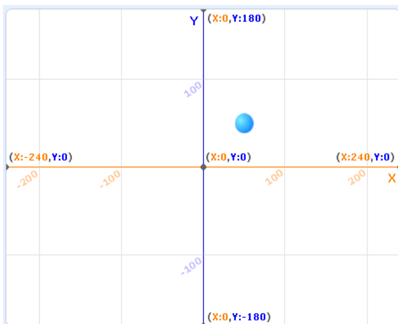
Figure 10: Rectangular Area
